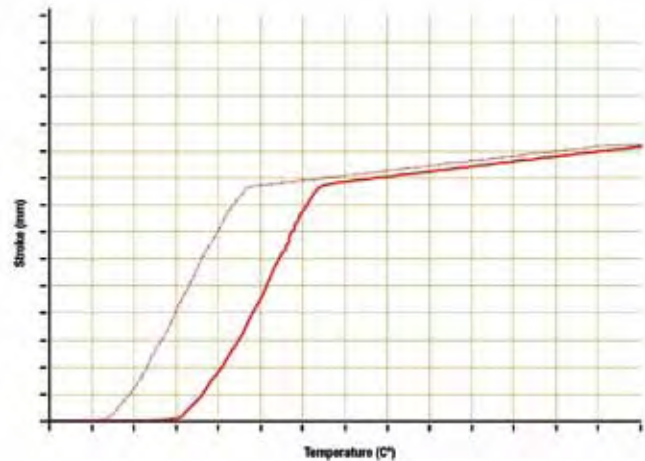
Displacement of the lid in function of the temperature of the FAE THERMOSTAT
